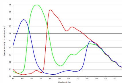
MV-CE200-11UC
